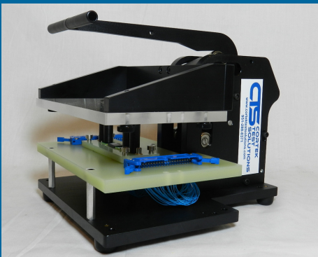
Flip top Mechanical Press for testing fine pitch contacts PCB.
