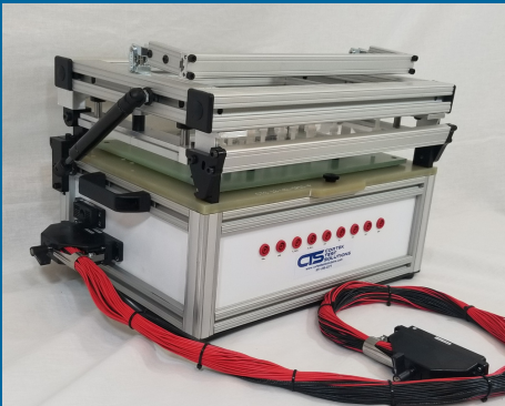
Z-Axis Mechanical Test Kit with custom programming and functional test fixture.
