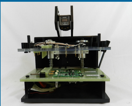
Mechanical Press with custom fixture for high volume production of automotive PCBAs.
